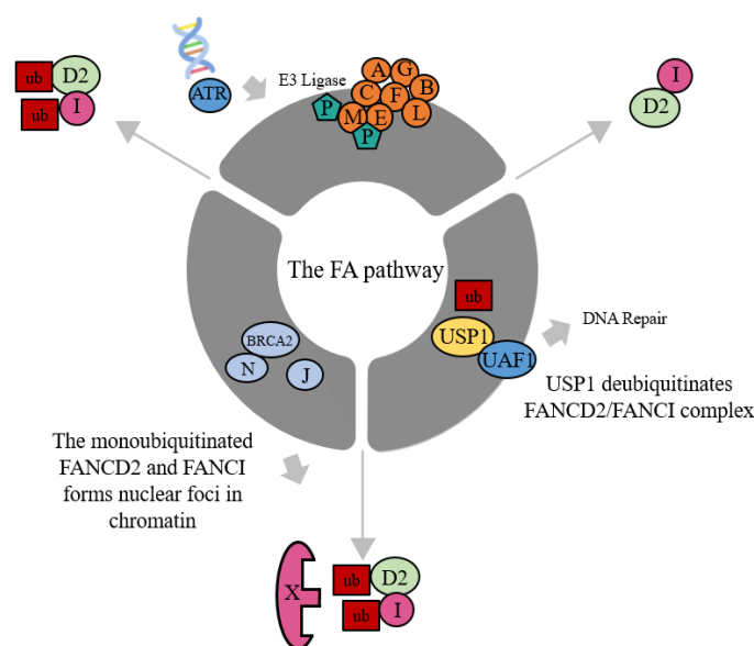
Figure 3. After DNA damage, the ATR kinase activates the FA core complex (Composed of FANCA/B/C/E/F/G/L/M). This complex acts as an E3 ubiquitin ligase, monoubiquitinating FANCD2 and FANCI. The monoubiquitinated FANCD2/FANCI complex then localizes to chromatin, where it interacts with other FA proteins and DNA repair factors. The USP1-UAF1 protein complex subsequently deubiquitinates FANCD2/FANCI, allowing their release from chromatin. Additionally, USP1 plays a role in directing FANCD2/FANCI to DNA repair foci.
