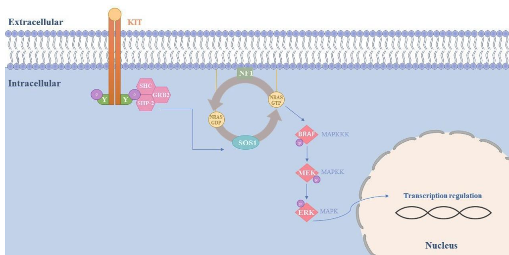
Figure 5. The MAPK signaling pathway is initiated by the conversion of GDP to GTP, activating Ras. Active Ras then binds and activates Raf, leading to the activation of MAPKKK. MAPKKK, also known as active Raf, further activates MAPKK, which in turn activates MAPK. The activated MAPK molecule moves to the nucleus, where it triggers the activation of diverse transcription factors.
